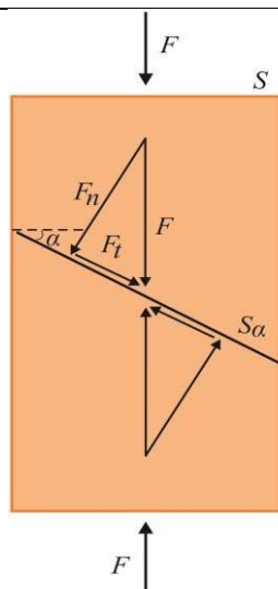
Rasm 2.3. Tashqi kuch ta'sirida kuchlanish holatini aniqlash uchun.
