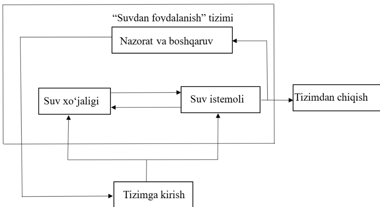
2-rasm. Suvdan foydalanishni dinamik tizim sifatida keltirish.
